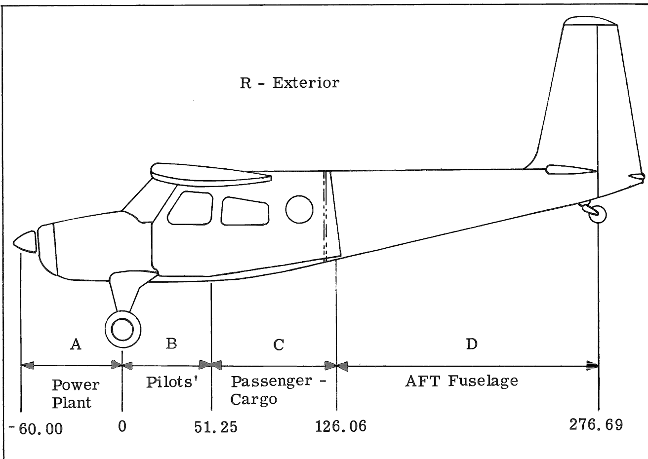
SECTIONAL BREAKDOWN
